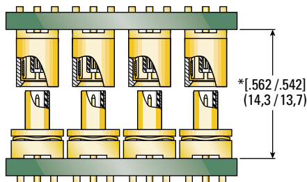
Stacked P.C. board configuration, using 3509-1511-000 and 3025-1511-011
