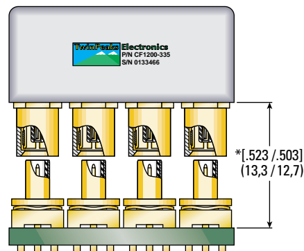
Modular component to P.C. board, using 3509-1511-000 and 3017-1511-005
