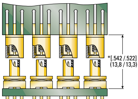
Daughterboard configuration, using 3509-1511-000 and 3025-1511-014 or -016
